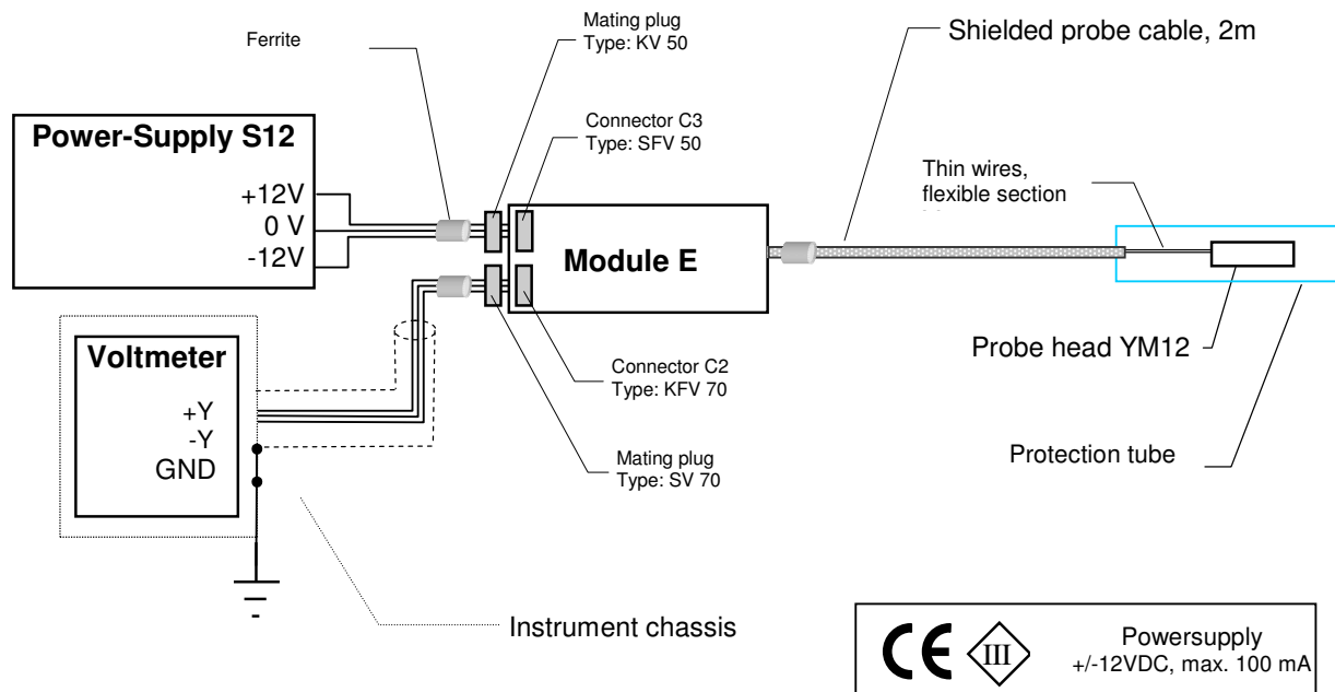
Figure 3: Set-up for all EMC-test
