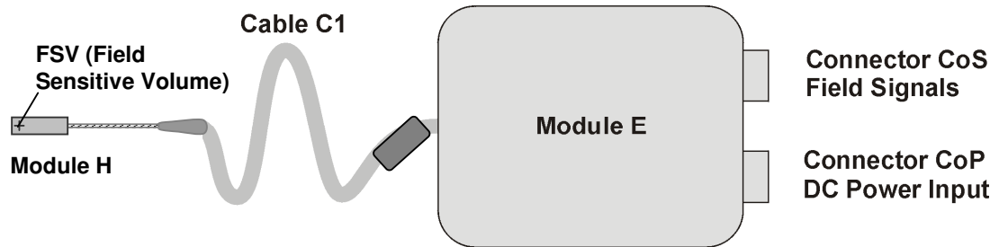
Figure 1: Structure of the Single-Axis Magnetic Field Hall Transducer YM12-3-2-0.2T
