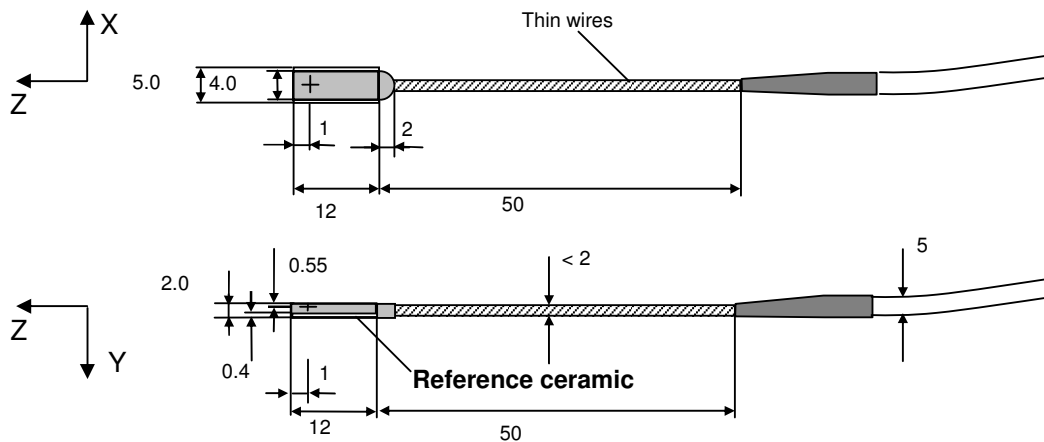
Figure 1: Structure of the Single-Axis Magnetic Field Hall Transducer YM12-3-2-0.2T
