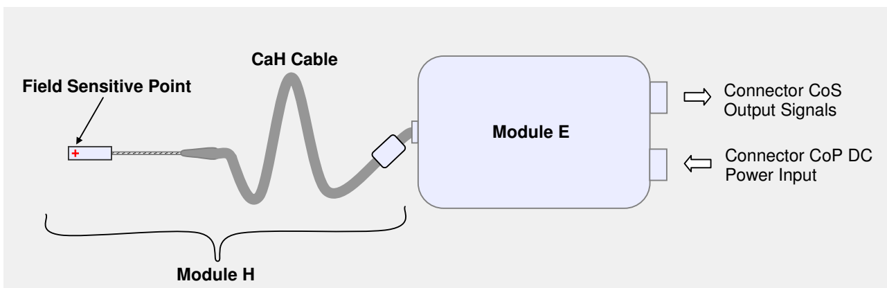
Figure 1: Schema of the SENIS low noise Hall Magnetic Field Transducer: - Module H, consisting of the Hall Probe and the CaH Cable - Module E, Analog electronics for signal conditioning. Note: The Cable CaH is permanently connected to the module E.
